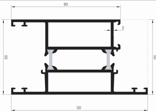
1065 T55 K 01 2,285 Kg/mt
