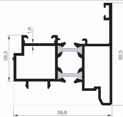
1066 T55 A 05 1,314 Kg/mt
