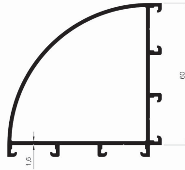
1055 RW60 A 04 1,166 Kg/mt
