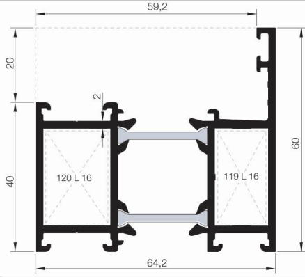
1067 T64 F 02 1,660 Kg/mt
