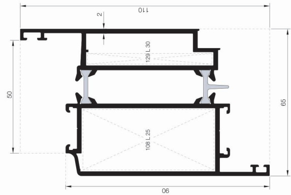
1062 T55 V 04 2,484 Kg/mt
