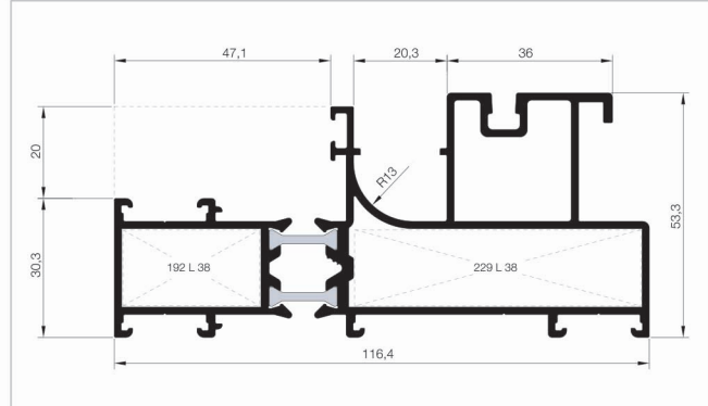
1076 T116 F 06 2,407 Kg/mt
