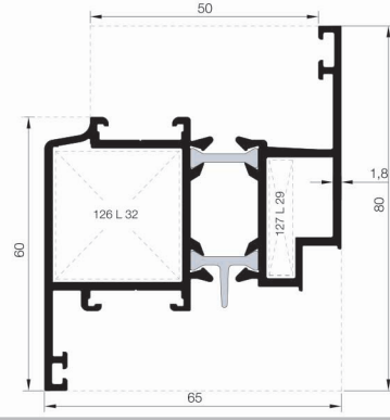
1060 T55 V 05 1,725 Kg/mt
