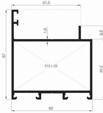
1052 RW60 V 01 1,162 Kg/mt
